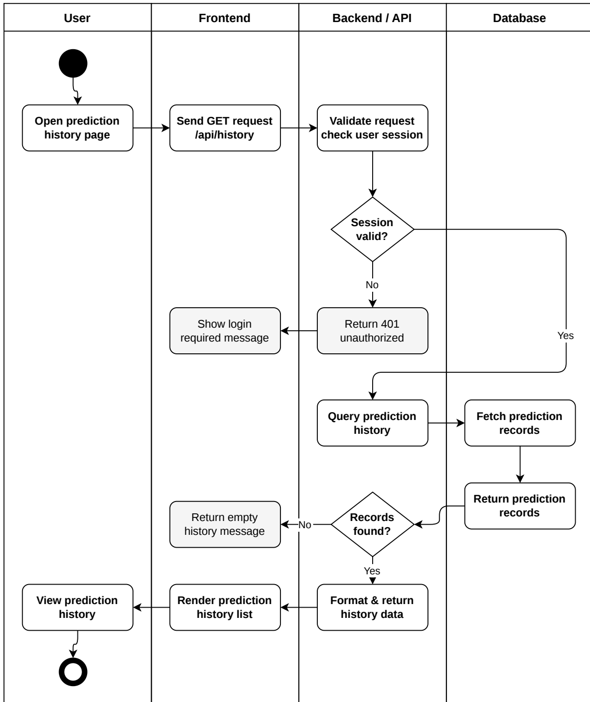
Activity Diagram — View Prediction History
